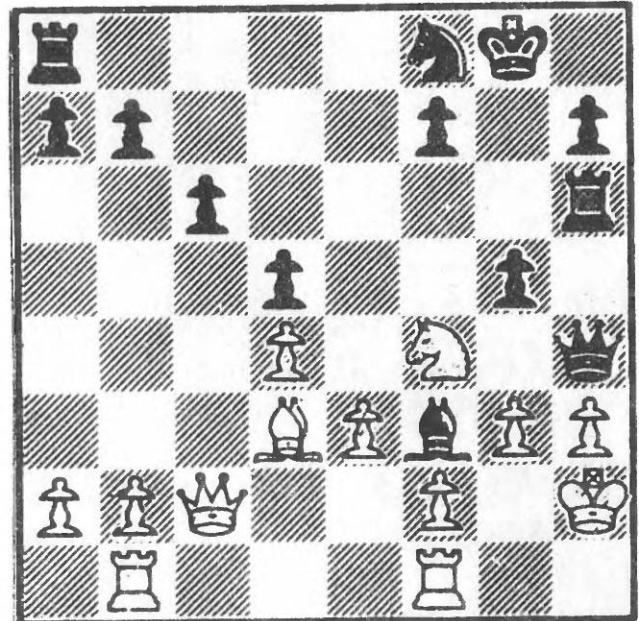
290 After 20 Kh2
